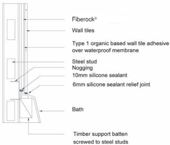
Bath Wall Junction Detail
