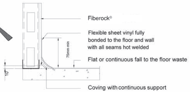
Wall to Floor Junctions Vinyl Floor Covering
