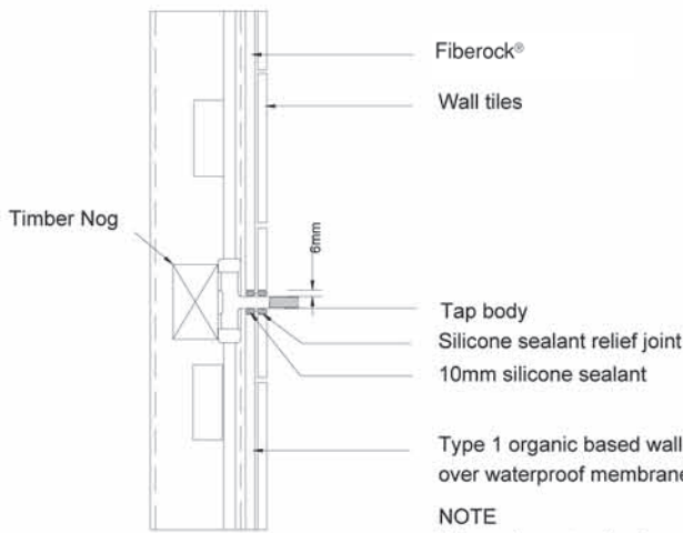
Typical Plumbing Penetration
