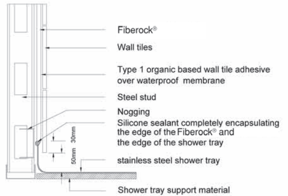
Shower Base Detail
