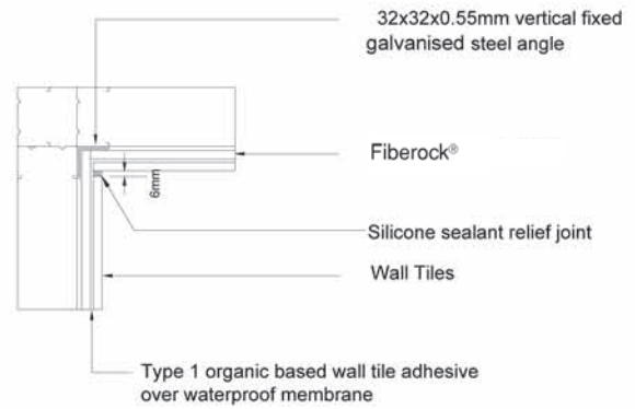
Tiled shower – Internal Corner Details
