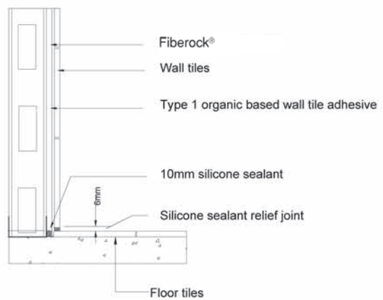
Wall to Floor Junctions Ceramic Tile Covering
