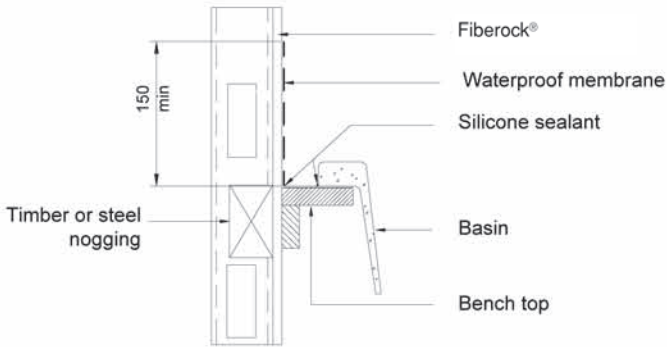
Tub, Sink and Basin
